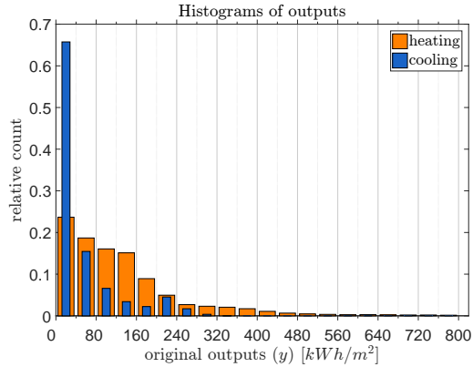
Figure 1: Distribution of the outputs y_n^{heating} for heating loads and y_n^{cooling} for cooling loads. The weight of the distributions is skewed towards lower values because we selected, unintentionally, more moderate climates (climates that need less cooling/heating or none) than extreme ones (need more heating, cooling, or both). Each building produces a slightly different distribution by itself – all simulations are plotted together here.
