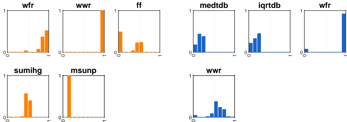
Figure 3: Histograms of the relevance parameters 1/l_i for significant input variables. A value of 1/l_i close to zero, for a particular input, indicates that that input was not involved in determining the prediction of the model. A significant input is one for which at least one non-zero value of 1/l_i has a relative share greater than 20% of the total samples. The group of plots on the left is for heating (orange), while on the right is for cooling (blue). The title of each plot is the variable code (see Table 2 for an explanation of the variable codes). The histogram is obtained from the 100 runs over training-data subsets of size N_{train} = 4,000 .
